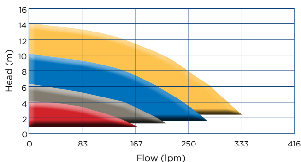
Supatuf MK2 ECO-V 100 Performance Curves
