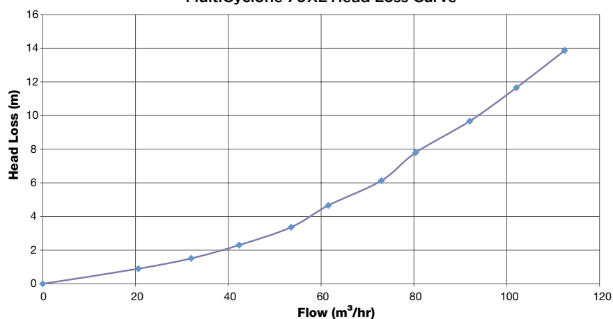
MultiCyclone 70XL Head Loss Curve
