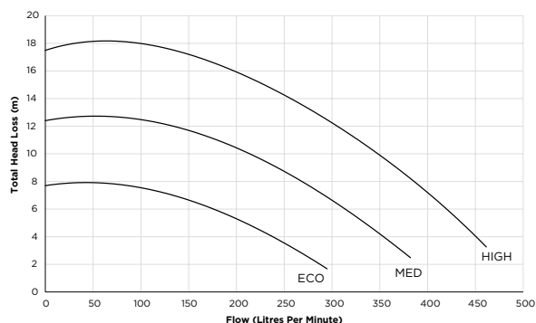
Alphaflo ECO-V 150 Performance Curves
