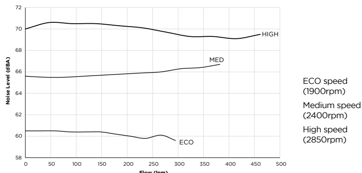
Alphaflo ECO-V 150 Noise Levels
