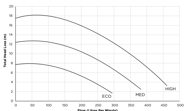
Alphaflo ECO-V 100 Performance Curves
