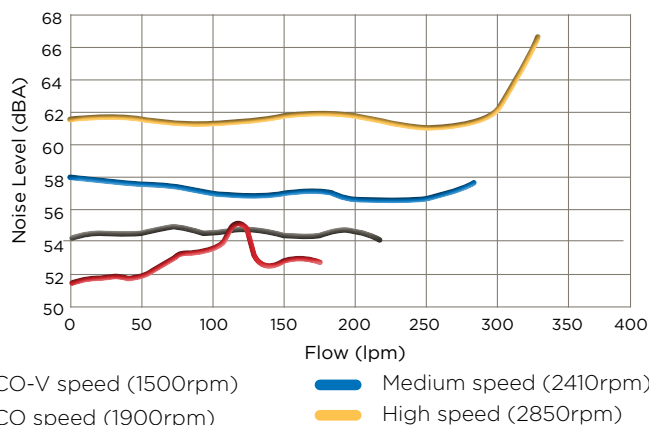
Supatuf MK2 ECO-V 100 Noise Levels
