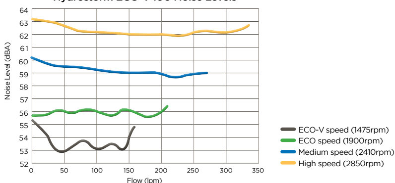
Hydrostorm ECO-V 100 Noise Levels
