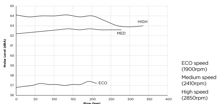
Alphaflo ECO-V 100 Noise Levels
