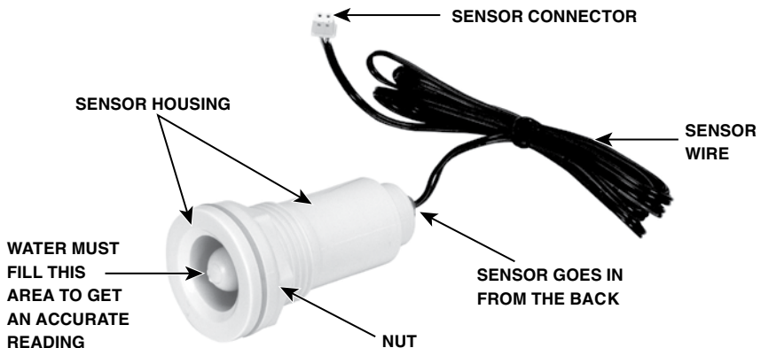
Figure 2: Temperature Sensor and Housing
